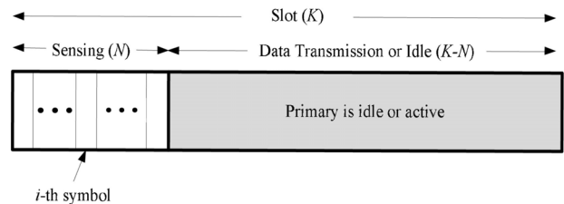
Fig. 1. Slot structure.
